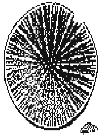
Solitary corals viewed normal to horizontal bedding, looking E
